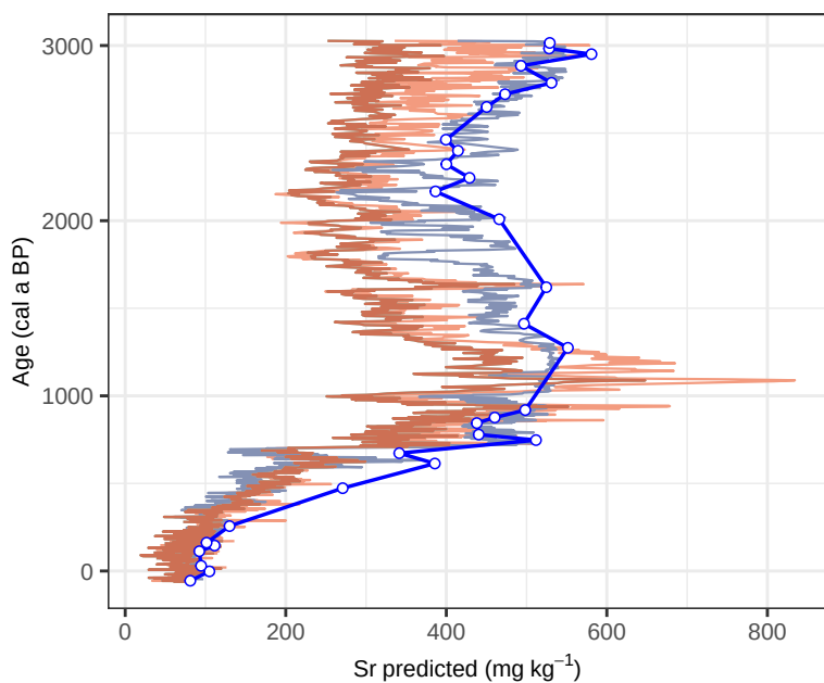
Site PB1 – Sr (age vs mg kg -1 , multivariate)
