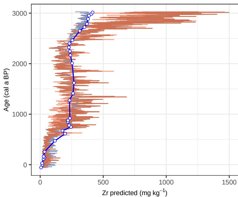
Site PB1 – Zr (age vs mg kg -1 , multivariate)
