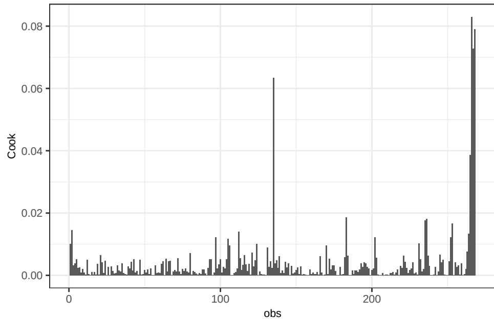
Zr WLS_weighted - Cook's Distance
