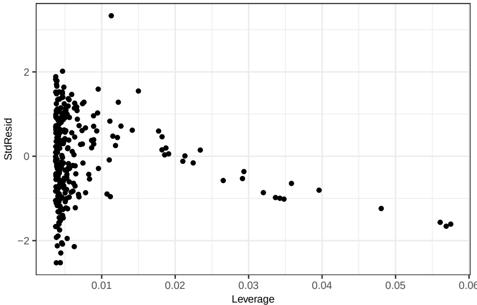
Zr WLS_weighted – Leverage Plot
