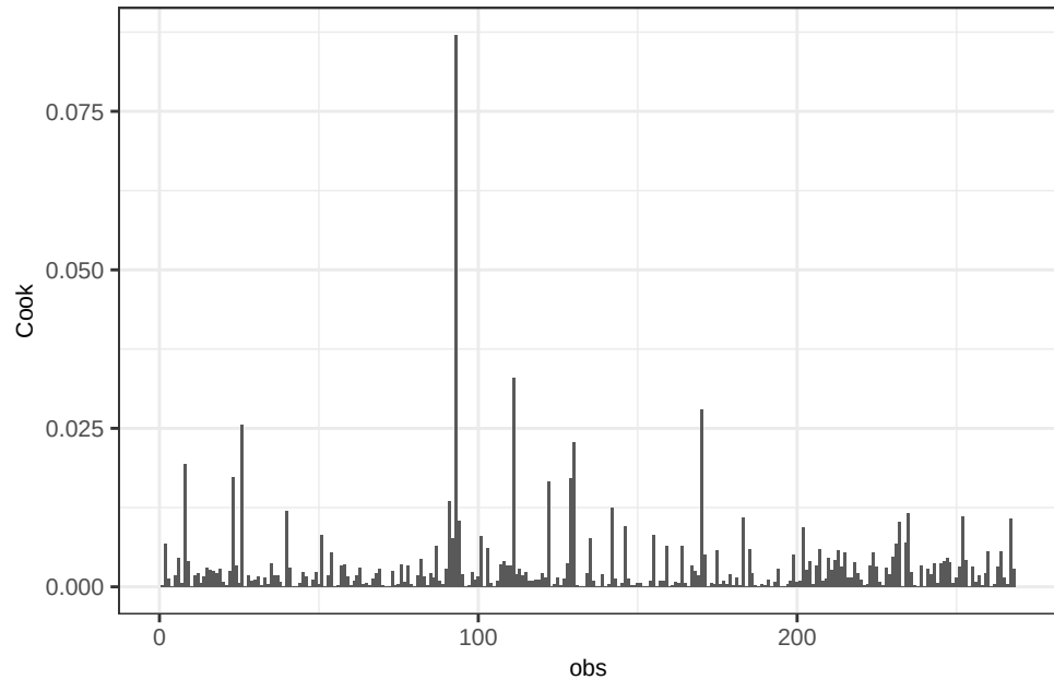
Mn OLS – Cook's Distance
