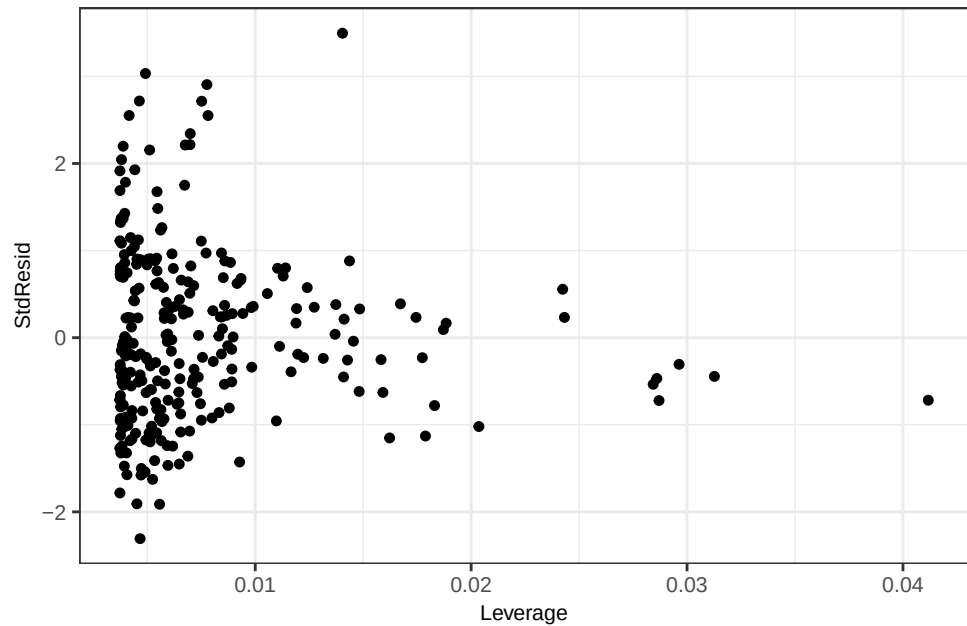
Mn OLS – Leverage Plot
