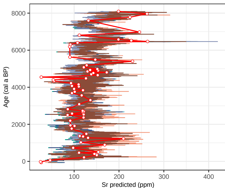
Site BI10 – Sr (age vs ppm, all)
