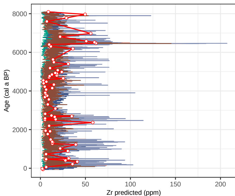
Site BI10 – Zr (age vs ppm, all)
