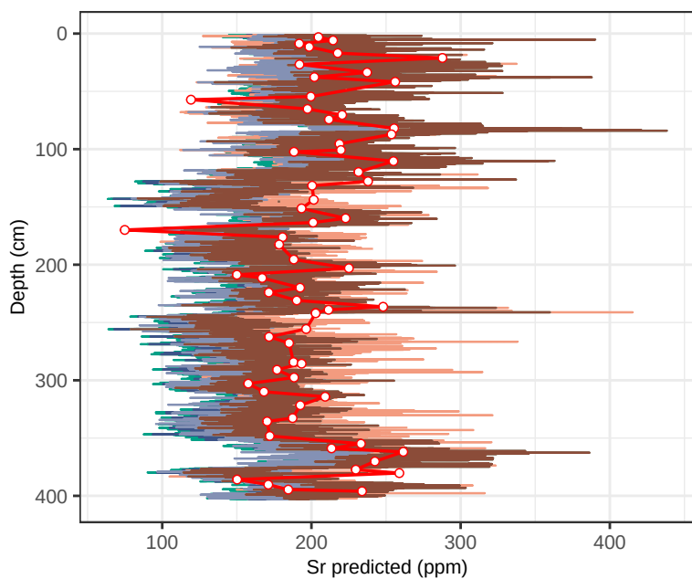
Site HER42PB – Sr (depth, all models)
