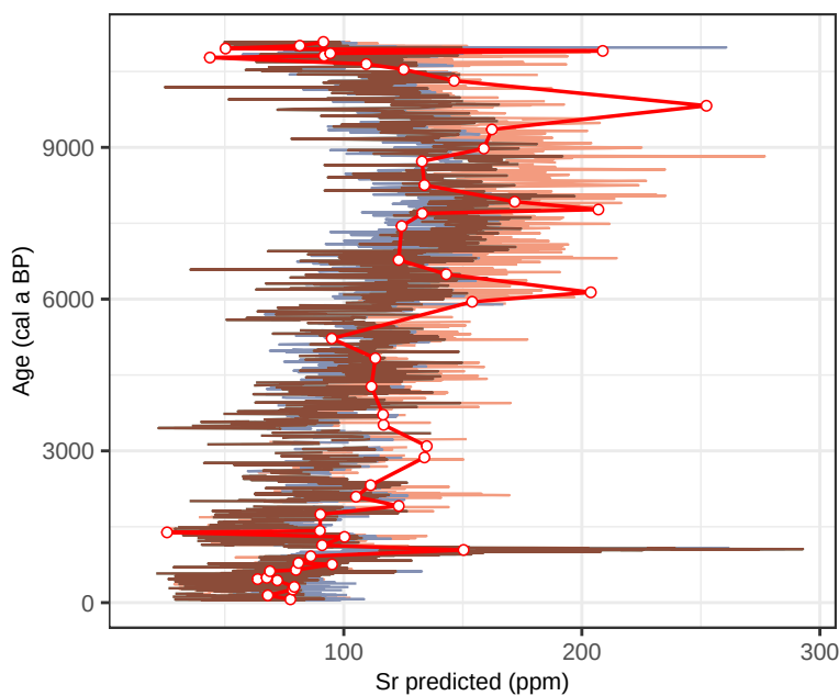
Site KER3 – Sr (age vs ppm, multivariate)
