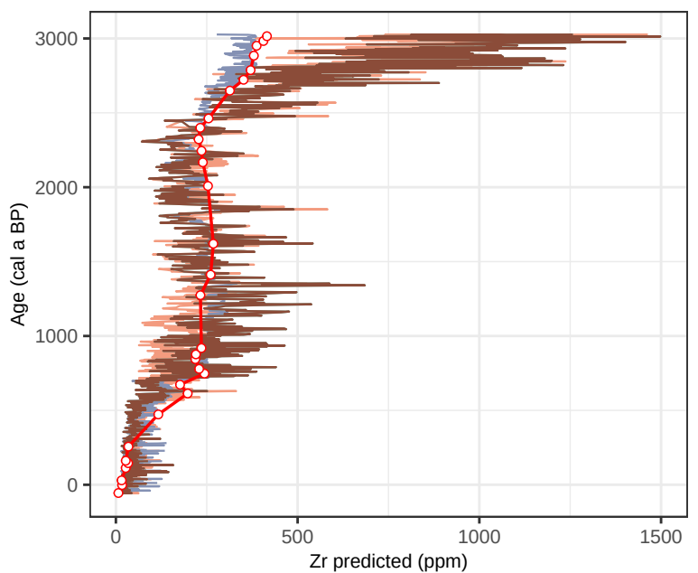
Site PB1 – Zr (age vs ppm, multivariate)
