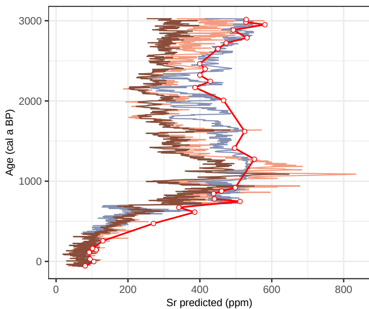
Site PB1 – Sr (age vs ppm, multivariate)
