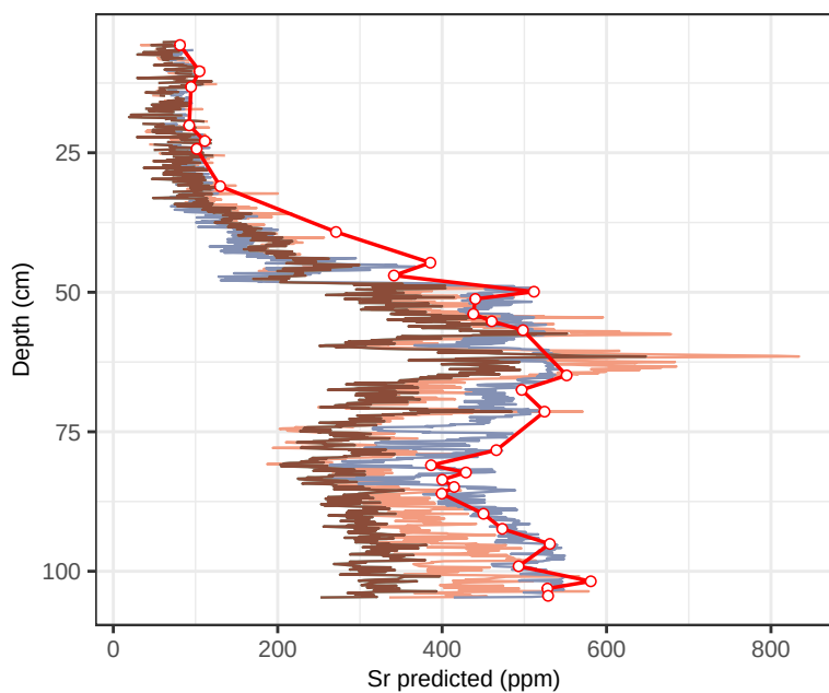
Site PB1 – Sr (depth, multivariate)
