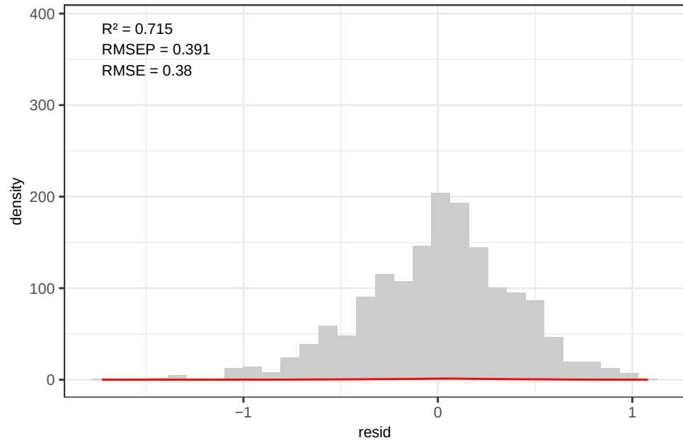
Ca - PLS(LOO) Residuals (log-space)
