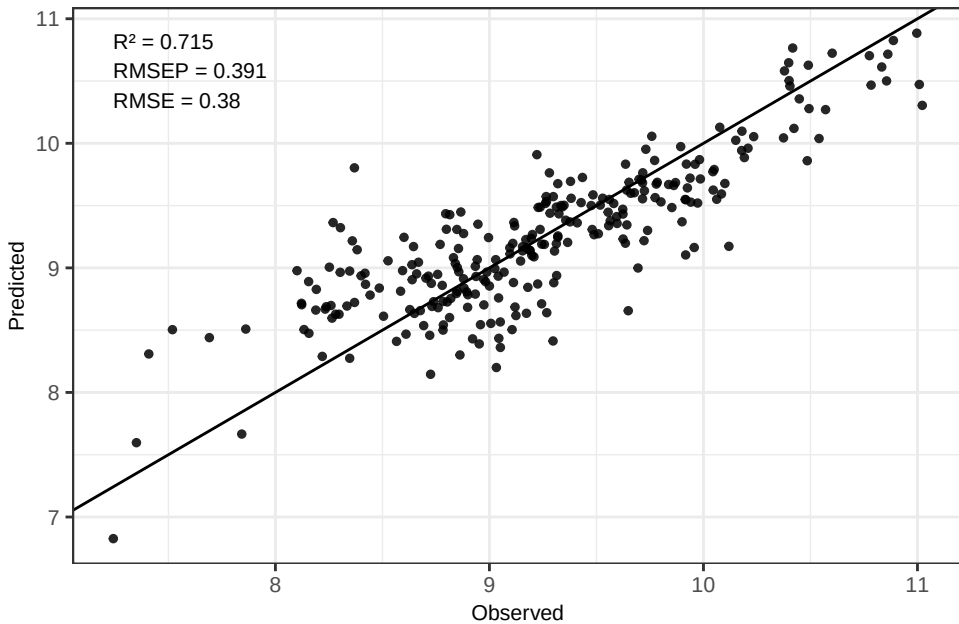
Ca - PLS(k) Predicted vs Observed (log-space)
