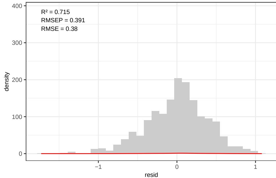
Ca - PLS(k) Residuals (log-space)
