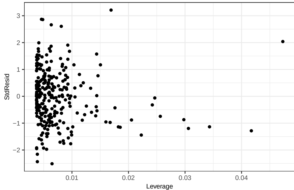
Fe WLS_weighted – Leverage Plot
