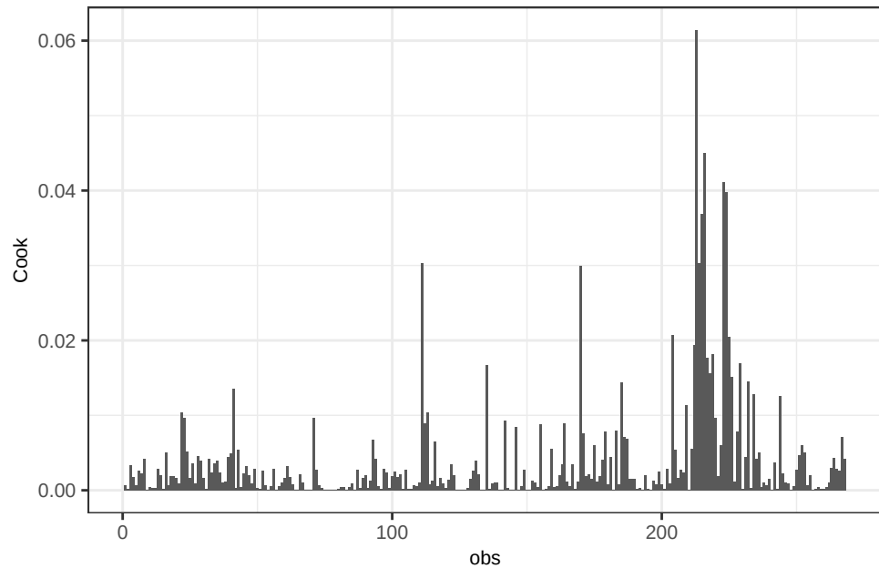
Fe - OLS(wt) Cook's distance
