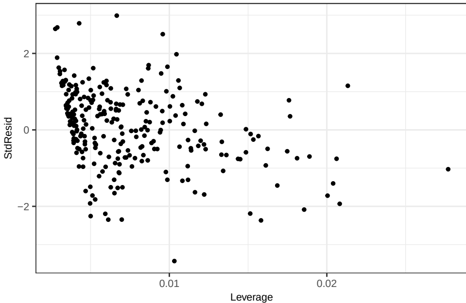
Fe - OLS(wt) Leverage vs Std. Residual
