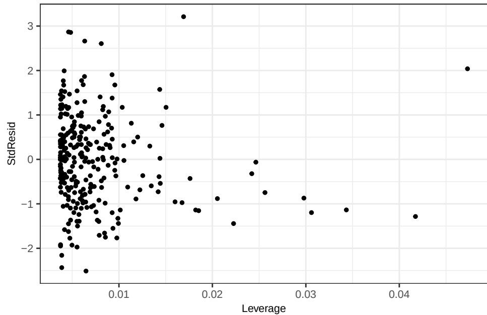
Fe - WLS(wt) Leverage vs Std. Residual
