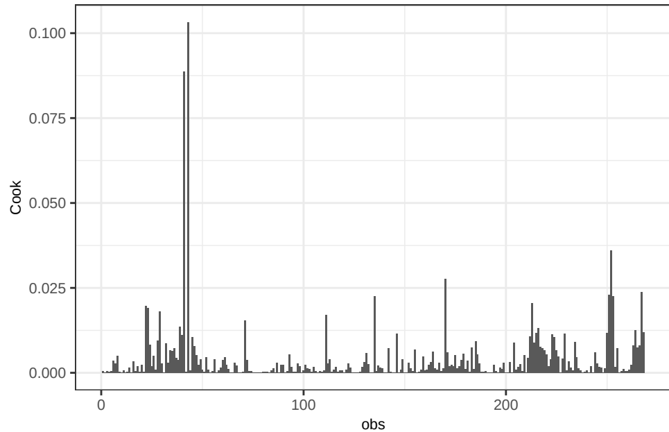
Fe - WLS(wt) Cook's distance
