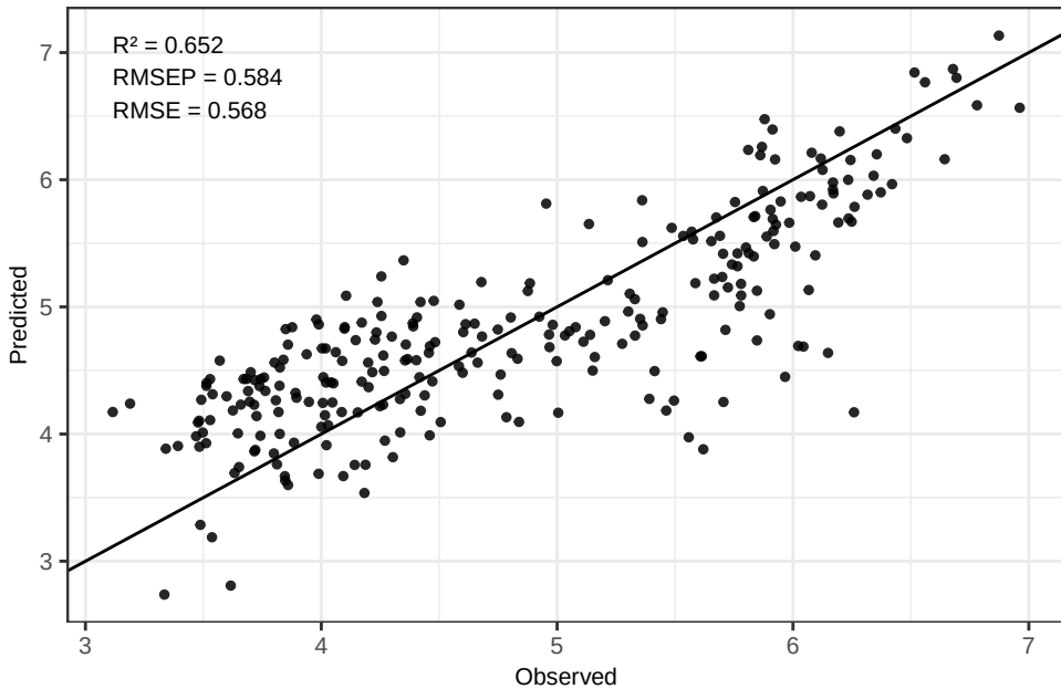
Mn - PLS(k) Predicted vs Observed (log-space)
