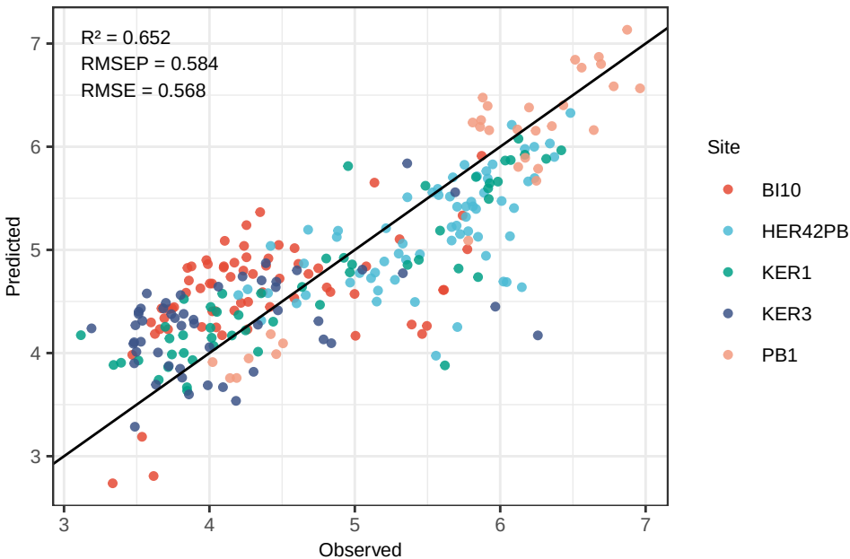
Mn PLS_LOO – Predicted vs Observed (log-space)
