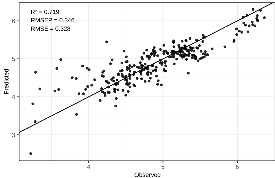
Sr - Bayes Predicted vs Observed (log-space)
