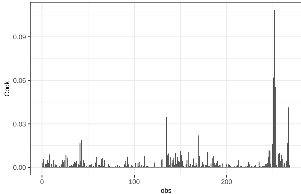
Ti - WLS(wt) Cook's distance
