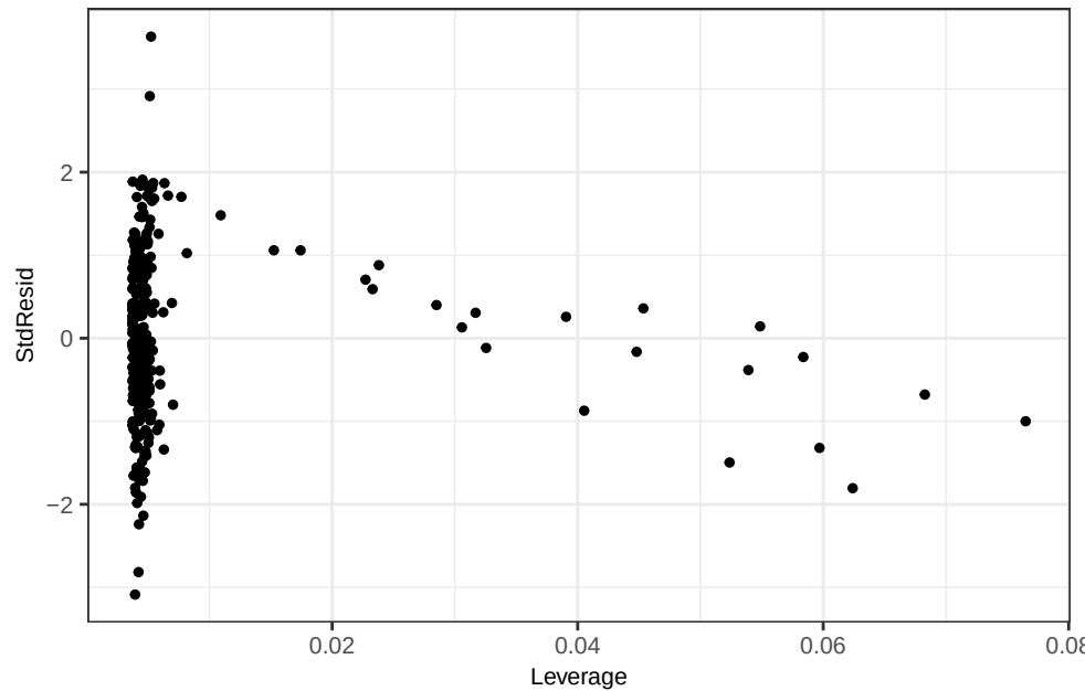
Ti - WLS(wt) Leverage vs Std. Residual
