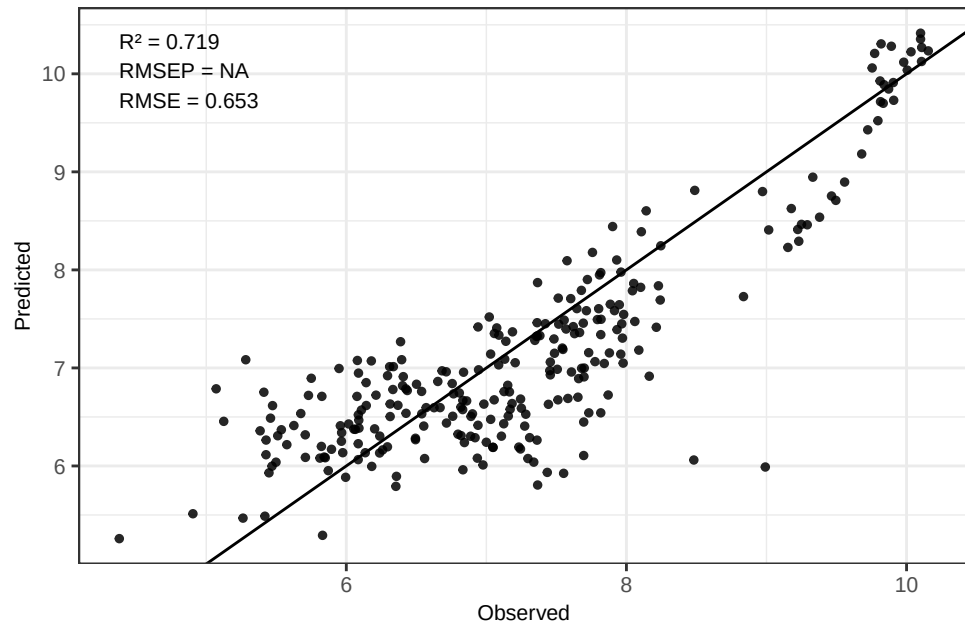
Ti – OLS(wt) Predicted vs Observed (log-space)
