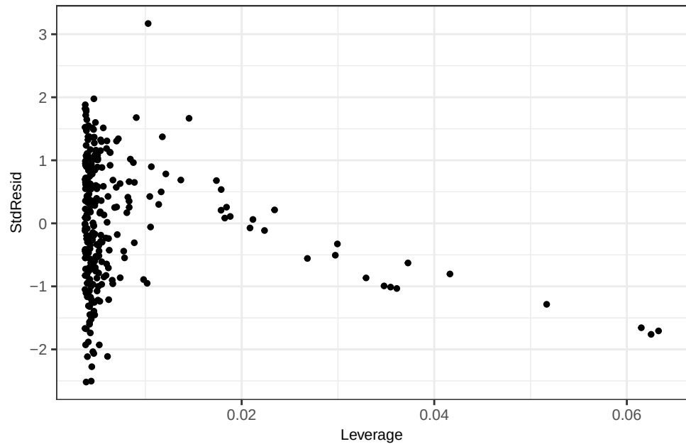
Zr – OLS Leverage vs Std. Residual
