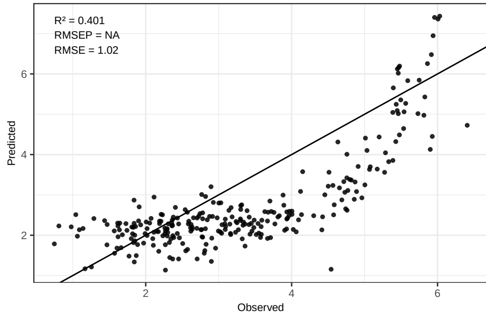
Zr – OLS(wt) Predicted vs Observed (log-space)
