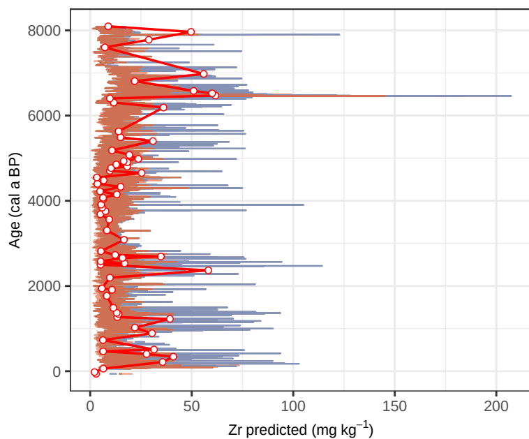
Site BI10 – Zr (age vs mg kg -1 , multivariate)
