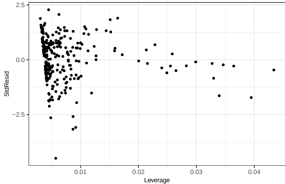
Ca - OLS(wt) Leverage vs Std. Residual
