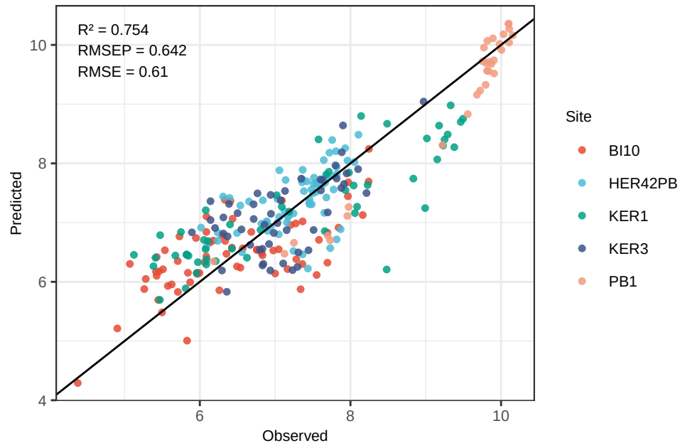
Ti PLS_kfold – Predicted vs Observed (log-space)
