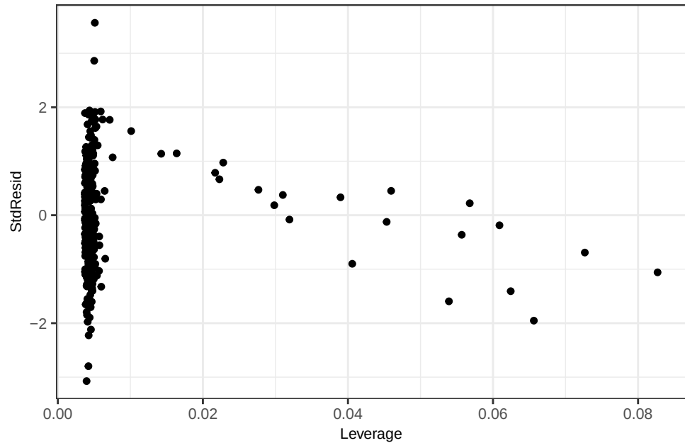
Ti WLS – Leverage Plot
