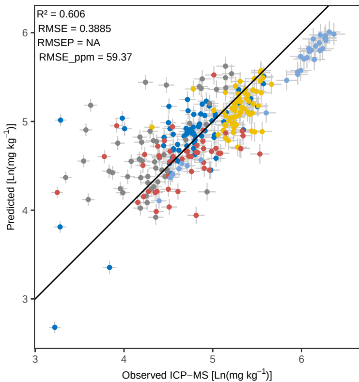
Sr WLS – Predicted vs Observed
