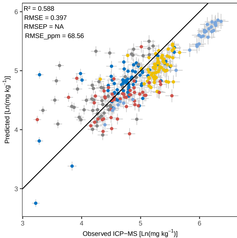
Sr OLS_weighted – Predicted vs Observed
