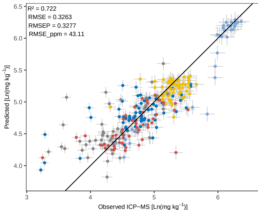
Sr RF – Predicted vs Observed
