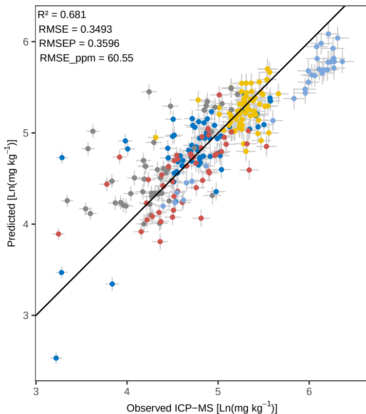
Sr PLS_LOO – Predicted vs Observed
