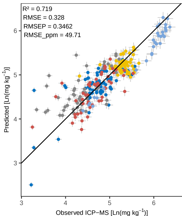
Sr Bayes – Predicted vs Observed
