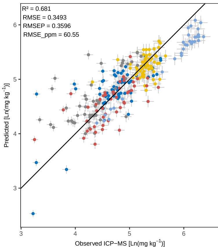
Sr PLS_kfold – Predicted vs Observed
