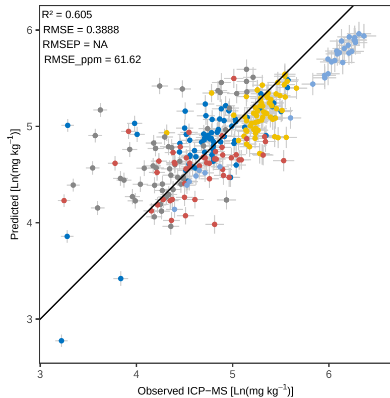
Sr WLS_weighted – Predicted vs Observed
