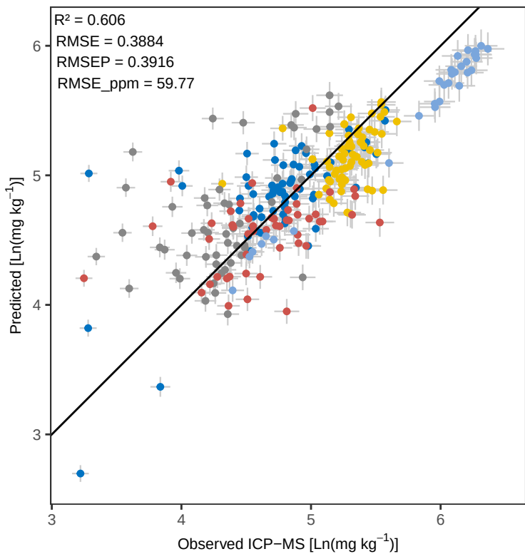
Sr OLS – Predicted vs Observed
