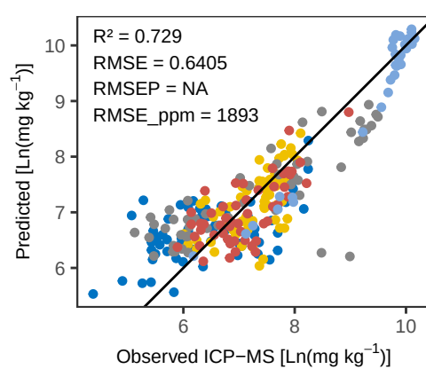
Ti RF – Predicted vs Observed (No Error Bars)
