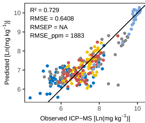
Ti Bayes – Predicted vs Observed (No Error Bars)
