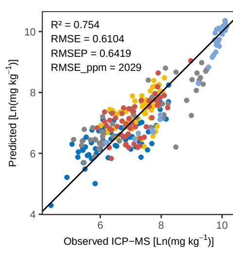
Ti PLS_LOO – Predicted vs Observed (No Error Bars)
