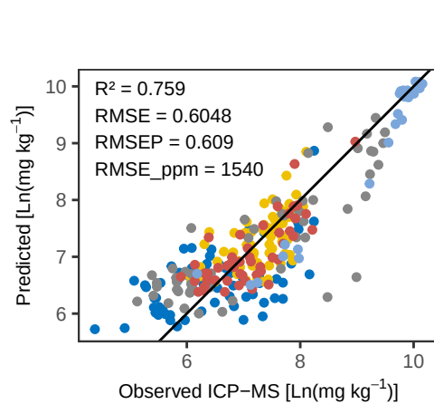
Ti RF – Predicted vs Observed (No Error Bars)
