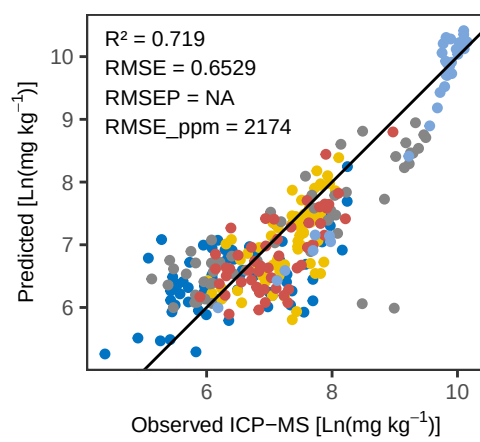
Ti WLS_weighted – Predicted vs Observed (No Error Bars)
