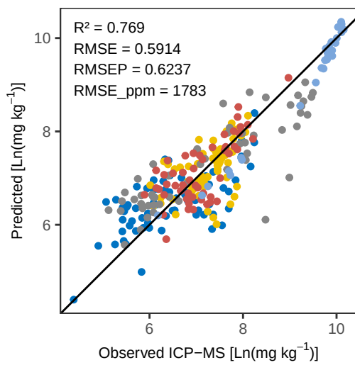
Ti PLS_kfold – Predicted vs Observed (No Error Bars)
