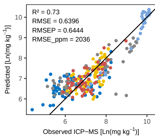
Ti WLS – Predicted vs Observed (No Error Bars)
