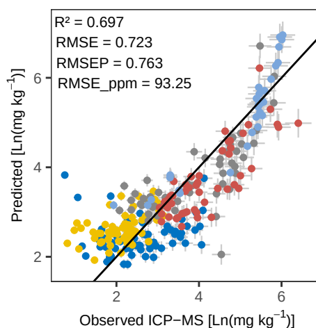
Zr PLS_LOO – Predicted vs Observed
