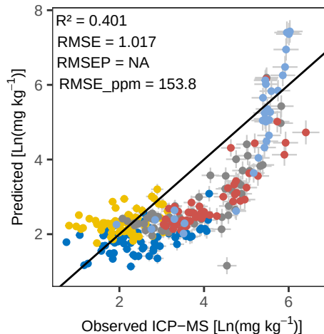
Zr WLS_weighted – Predicted vs Observed
