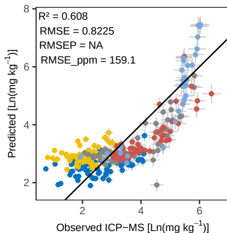
Zr Bayes – Predicted vs Observed
