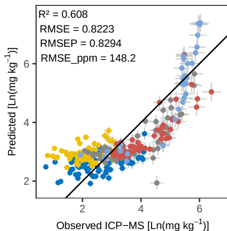
Zr WLS – Predicted vs Observed
