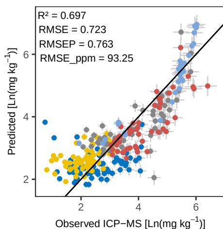
Zr PLS_kfold – Predicted vs Observed
