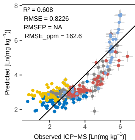
Zr RF – Predicted vs Observed
