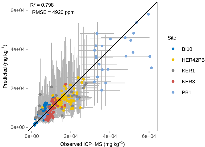
Ca Bayes – ACE Pred vs Ob (abs err)
