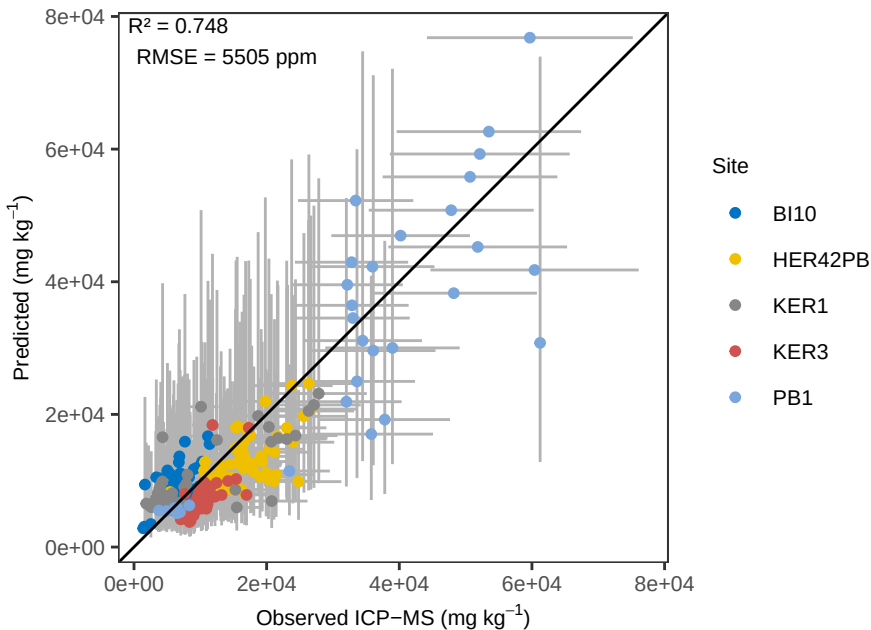
Ca OLS – ACE Pred vs Ob (abs err)
