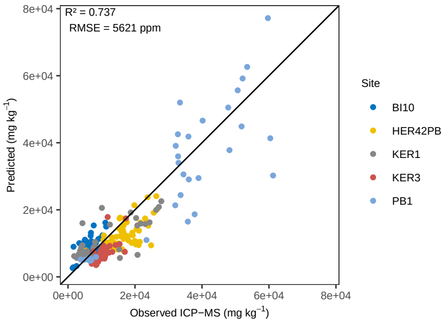
Ca OLS_weighted – ACE Pred vs Obs
