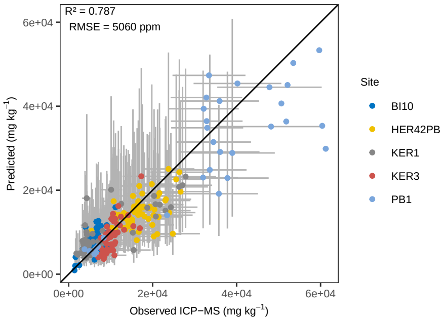
Ca PLS_LOO – ACE Pred vs Ob (abs err)
