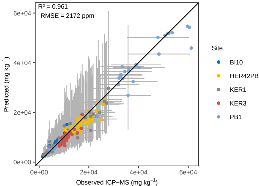
Ca RF – ACE Pred vs Ob (abs err)
