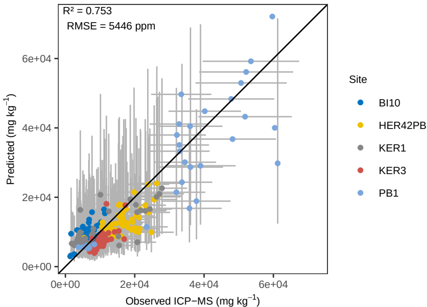
Ca WLS – ACE Pred vs Ob (abs err)
