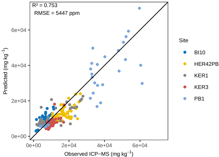
Ca WLS_weighted – ACE Pred vs Obs
