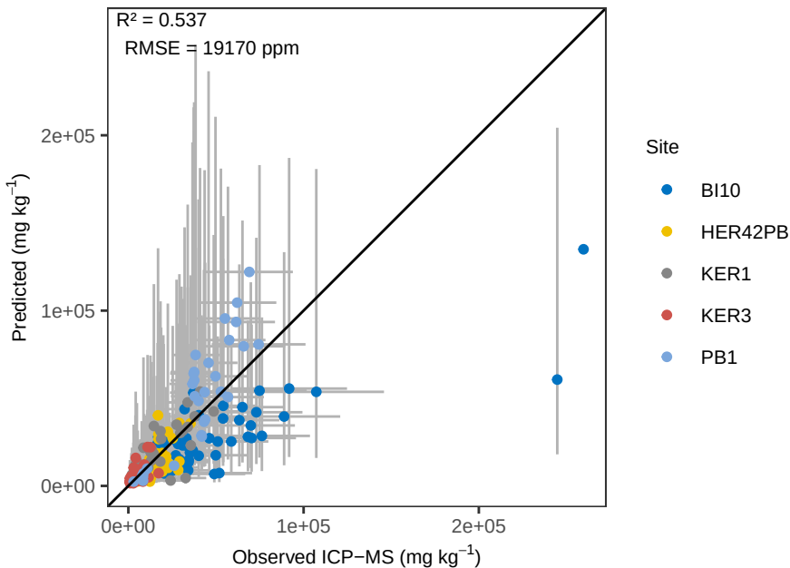
Fe OLS_weighted – ACE Pred vs Ob (abs err)
