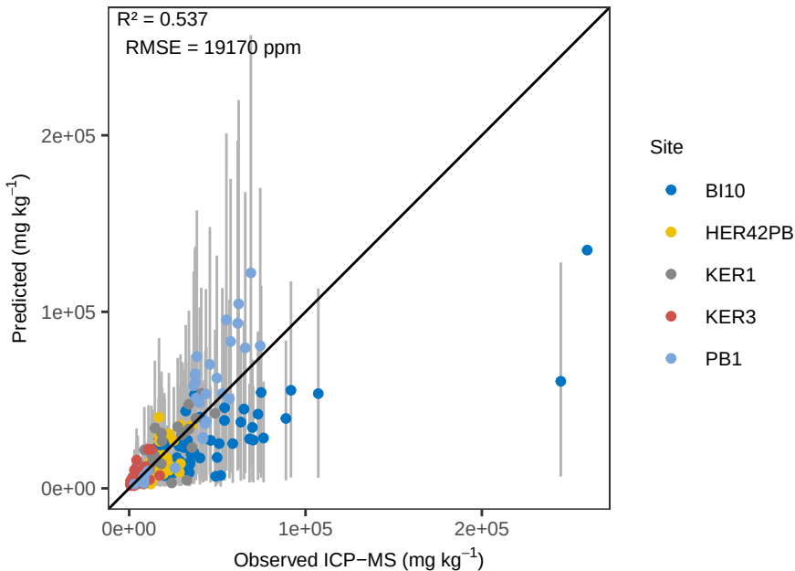
Fe OLS_weighted – ACE Pred vs Ob (% err)
