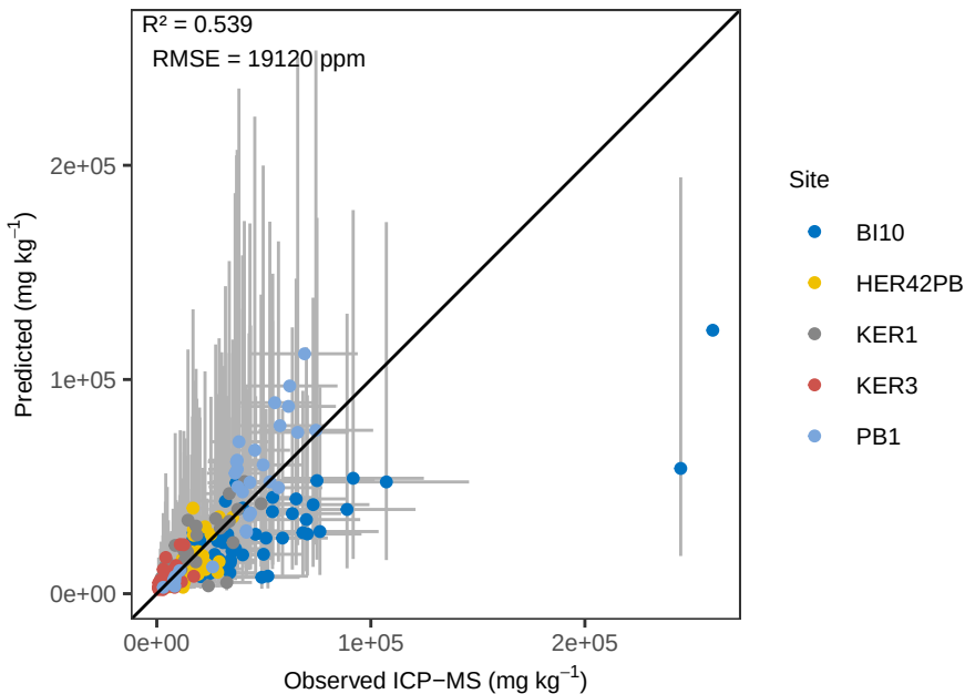
Fe WLS_weighted – ACE Pred vs Ob (abs err)
