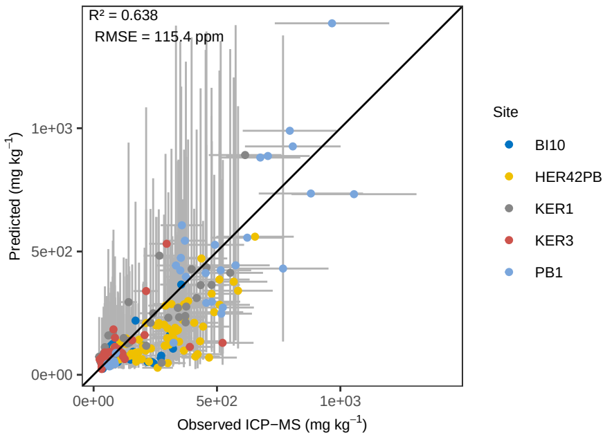
Mn OLS_weighted – ACE Pred vs Ob (abs err)
