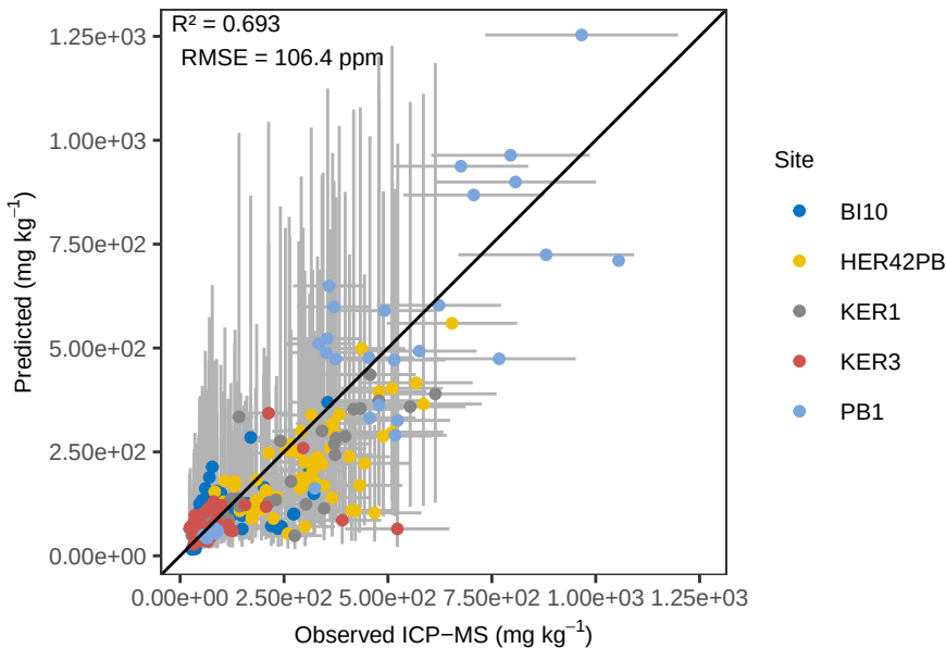
Mn PLS_LOO – ACE Pred vs Ob (abs err)
