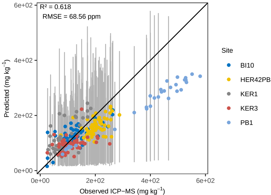
Sr OLS_weighted – ACE Pred vs Ob (% err)
