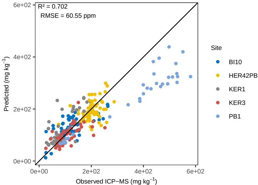
Sr PLS_kfold - ACE Pred vs Obs
