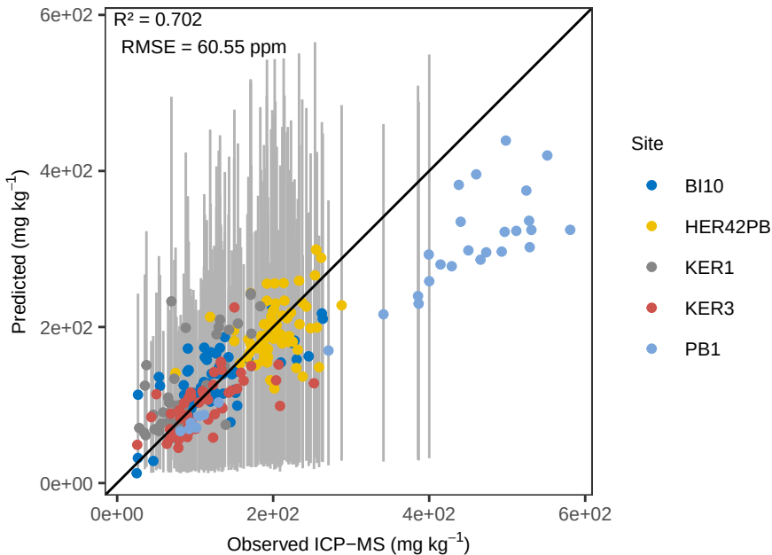
Sr PLS_kfold – ACE Pred vs Ob (% err)
