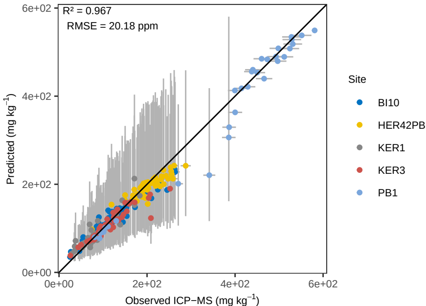
Sr RF – ACE Pred vs Ob (abs err)
