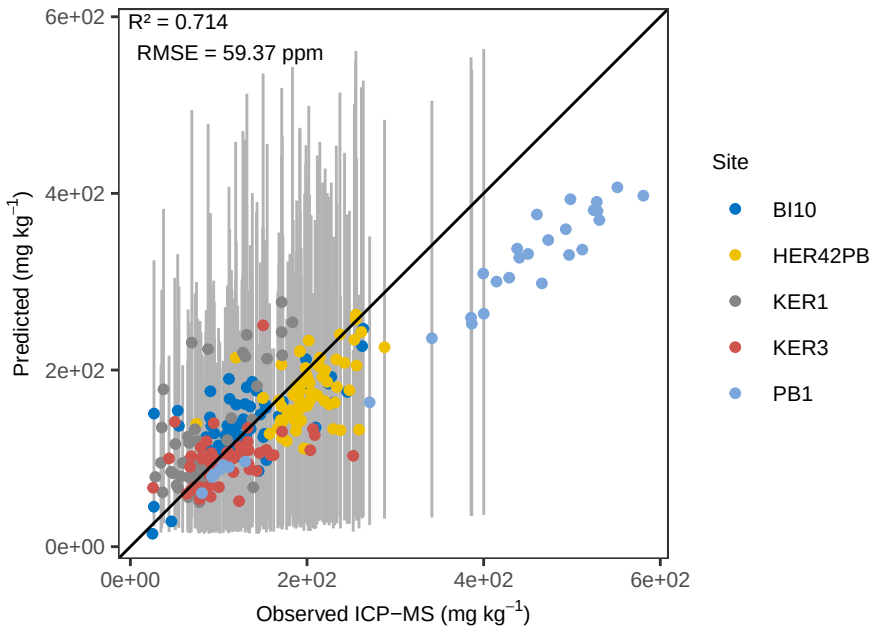
Sr WLS – ACE Pred vs Ob (% err)
