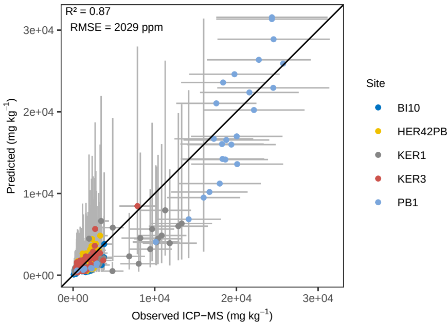
Ti PLS_kfold – ACE Pred vs Ob (abs err)
