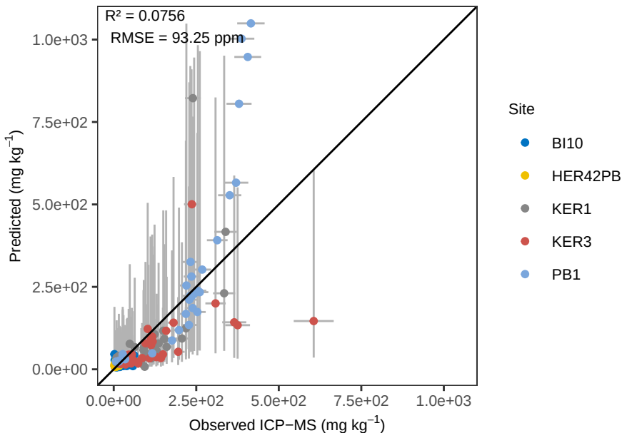
Zr PLS_kfold – ACE Pred vs Ob (abs err)
