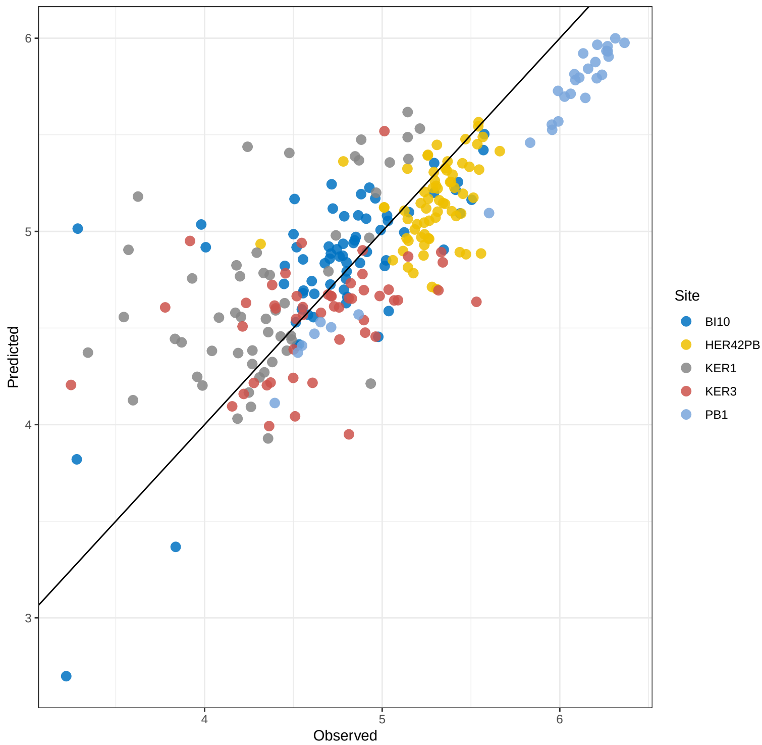
Sr PLS_kfold – Predicted vs Observed
