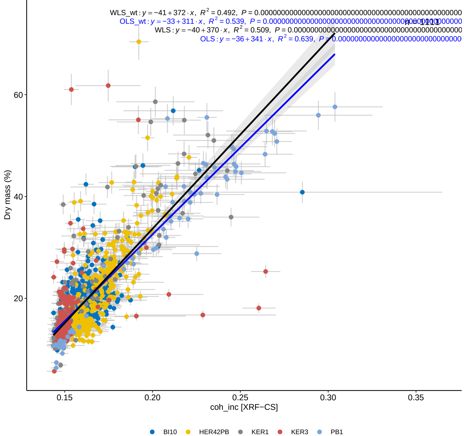
Site: ACE : Dry mass vs coh_inc
