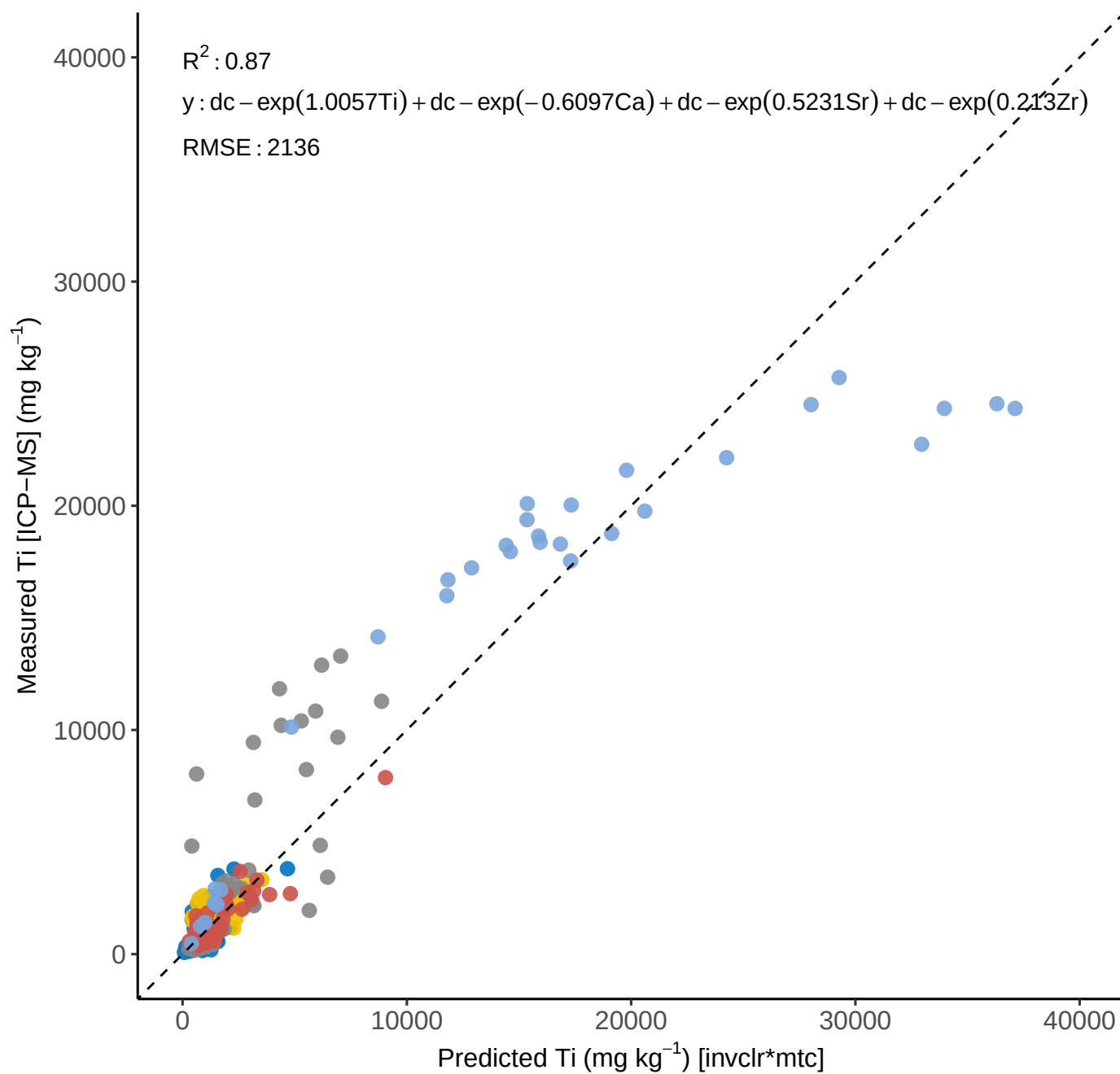
PLS Ti log_inc model as \text{mg kg}^{-1}
